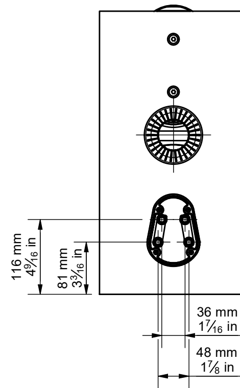
REAR
