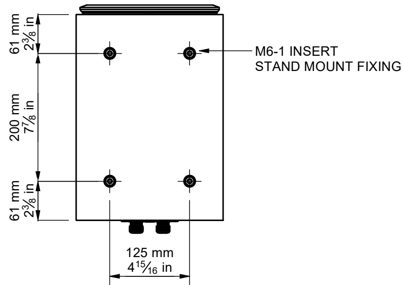
BASE
