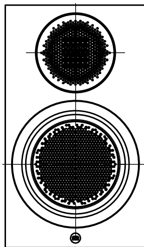
FRONT - GRILLE OFF
