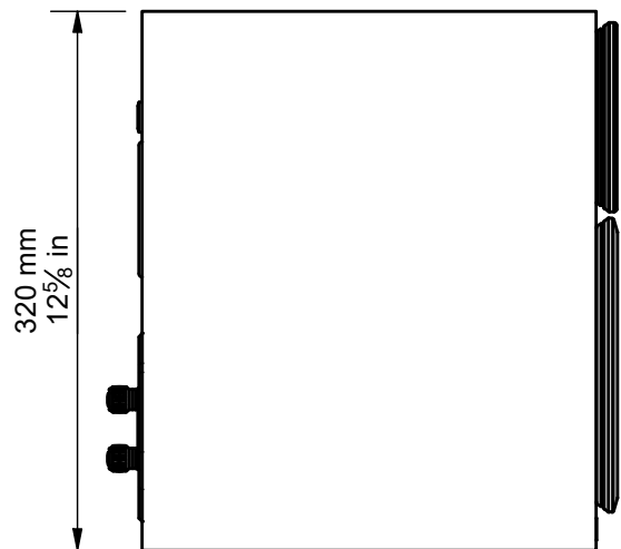
SIDE - GRILLE ON
