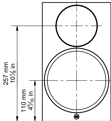
FRONT - GRILLE ON
